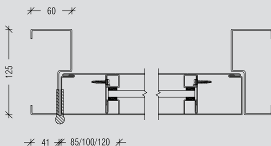
SINGLE DOOR SECTION
