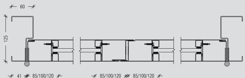
INTEGRAL ASTRAGAL DETAILS
